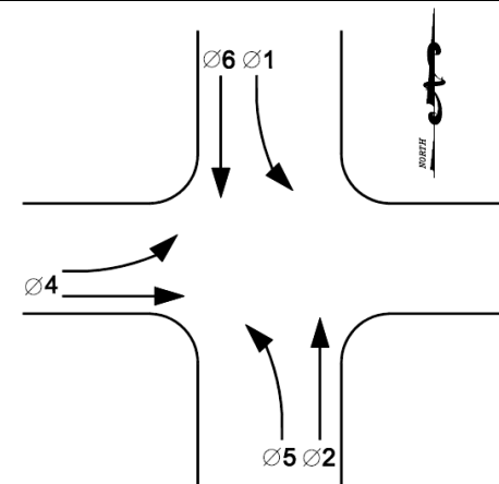
Figure: Signal Phasing ( \phi ) Diagram
